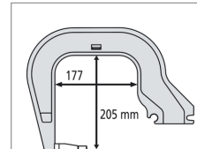
Bras C3 8 bar/550 daN
